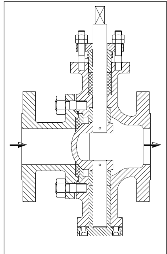
V-NOTCH BALL VALVE
