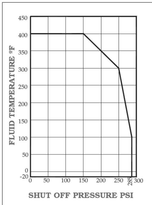
PRESSURE / TEMPERATURE FOR PTFE BALL SEALS
