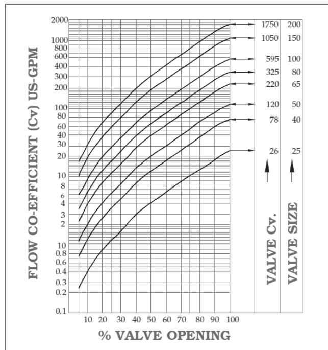
FLOW CHARACTERISTIC CURVES 90° OF OPENING
